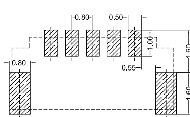
Recommended P.C.B Layout General Tolerance±0.05
